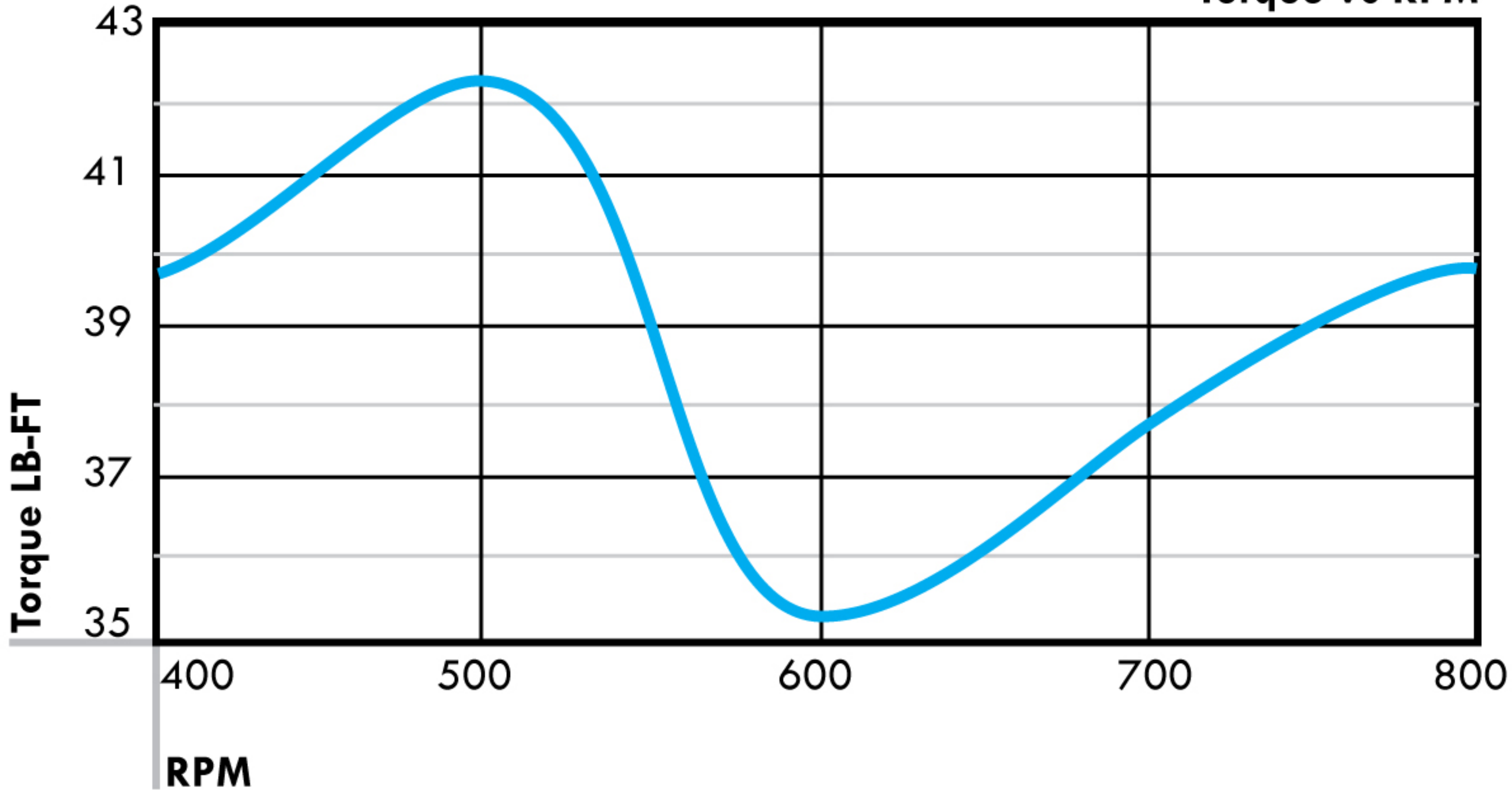
Torque vs RPM
